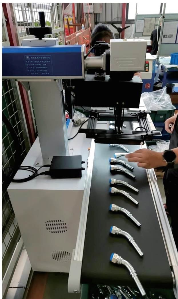
Automatic laser marking machine
